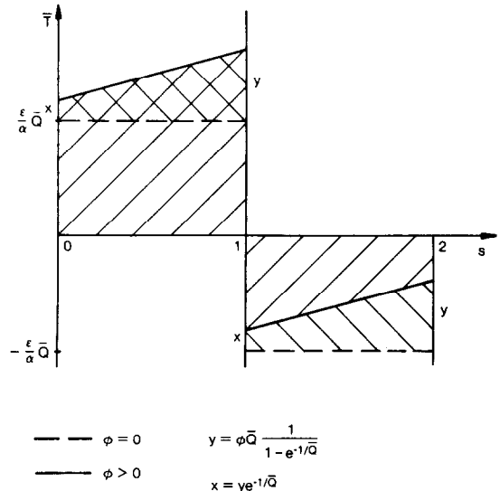
FIG. 3. The temperature distribution in the first loop.
